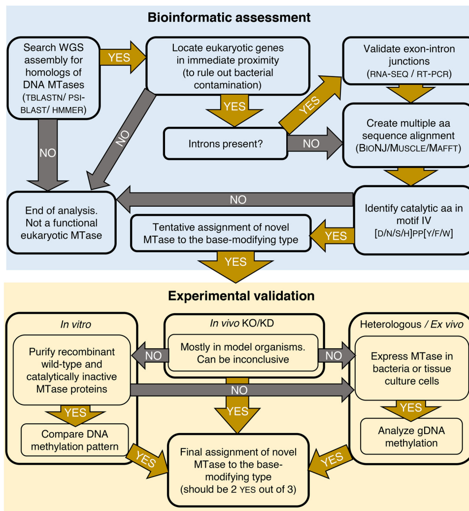
FIGURE 3 A flowchart outlining the required steps in identification and validation of novel DNA amino-MTases in eukaryotic genomes. WGS, whole-genome sequence; aa, amino acid. The [DNSH]PP[YFW] amino acid string in motif IV can serve as an initial indicator: most N4C-MTases have the SPPY catalytic string, while most N6A-MTases feature DPPY that distinguishes them from eukaryotic N6AMT1 (NPPY, N 5 -Gln), N6AMT2 (DPPY/F, N 5 -Lys), or METTL4-like enzymes (DPPW, also seen in METTL3/IME4-like m 6 A-RNA MTases).
