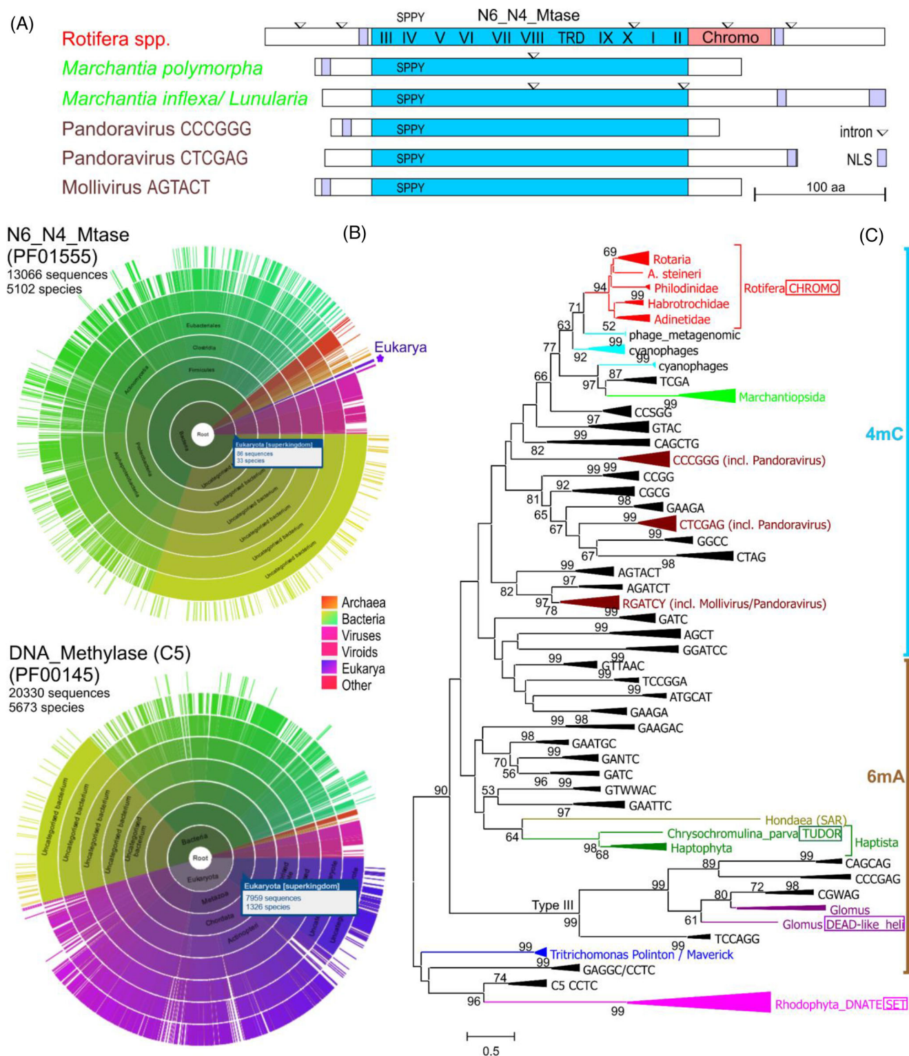
FIGURE 2 Domain structure and distribution of N6_N4_MTases. (A) Structural organization of eukaryotic N4C-MTases from rotifers, liverworts and giant viruses. Shown are conserved motifs I-X in the permuted MTase domain, intron positions (triangles), and nuclear localization signals (NLS) predicted via HMM. [128] (B) Visualization of PF01555 distribution across species as a “sunburst” diagram from PFAM, with each ring (from inside to outside) showing the number of taxa within superkingdom, kingdom, phylum, class, order, family, genus, and species, respectively. The eukaryotic sector is marked with a purple asterisk. For comparison, the analogous distribution of PFAM family members for PF00145 (C5 DNA_methylase) is shown below. HMM search details are outlined in Table S1. (C) Clustering of eukaryotic MTases (in color) with their prokaryotic counterparts (in black) by the neighbor-joining algorithm. Prokaryotic MTases with their recognition sequences are from REBASE. N4C-MTases from bdelloid rotifer families, red; from liverworts, lime green; giant virus N4-MTases (in brown) are nested within the respective bacterial groups; cyanophages are highlighted in cyan. N6A-MTases from SAR, Haptista and Fungi are in olive, green, and purple, respectively. Putative parabasalid
